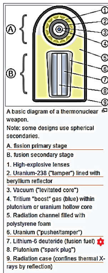
Figure 1. A Diagram of a Thermonuclear Device showing beryllium, lithium and uranium components. Asterisk indicates that modern devices use natural lithium. A natural mixture of 95% Li7 and only 5% Li6 nuclear isotopes as was first demonstrated in the Castle Romeo Test [4]. Figure adapted from Wikipedia Commons.
