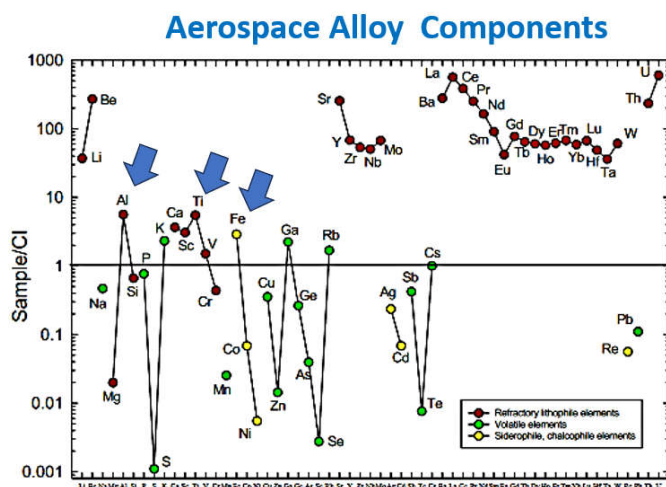
Figure 4. The Ti Al Fe elemental abundances of Spherule 21 (Normalized to CI Chondrites) versus atomic number for 56 elements. The Solar System standard of CI chondrites is represented by a value of unity on the plot. Elements often associated with high strength aerospace alloys are indicated by blue arrows. Nickel, which like iron is an end product of nucleosynthesis in the majority of stars, is of very low abundance in this sample relative to iron, indicating this sample is not derived from a planetary molten core.
