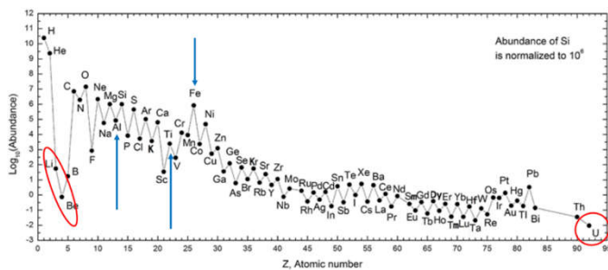
Figure 2. Graph of Log 10 relative abundance versus Si in CI carbonaceous Chondrites whose relative elemental abundances have been found to match those in the found in the Sun. Note the close values for abundance of Nickel and Iron.
