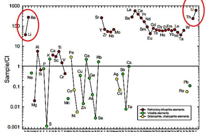
Figure 3. The "BeLaU" elemental abundances of Spherule 21 (Normalized to CI Chondrites) versus atomic number for 56 elements. The Solar System standard of CI chondrites is represented by a value of unity on the plot. Elements seen to be associated in Thernuclear devices are circled in red.
